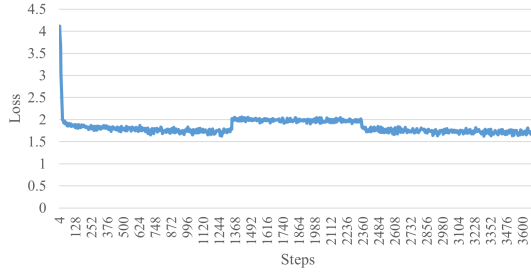
Fig. 3. Training loss curve during the fine-tuning stage.
