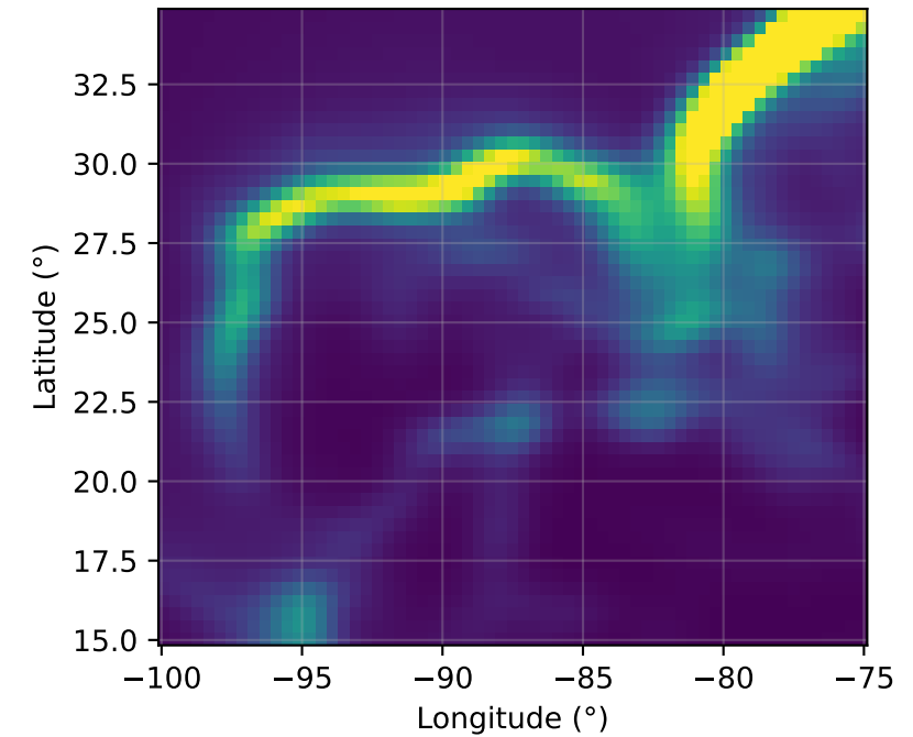
Predicted S_T : Laplace-fill
