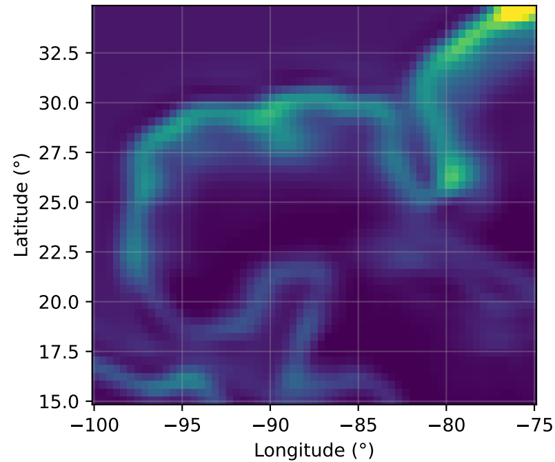
Predicted S_T : Zero-fill
