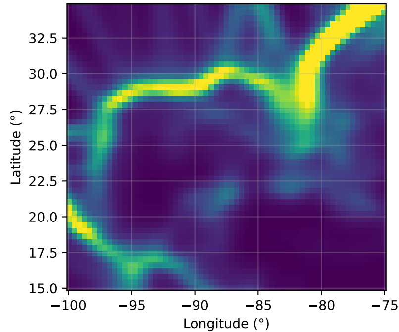
Predicted S_T : Replicate-fill
