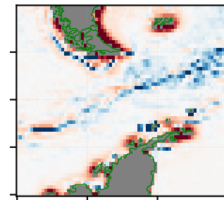
(f) mean_fill
