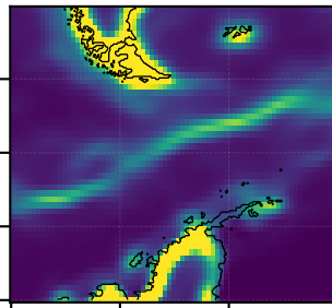
(f) mean_fill
