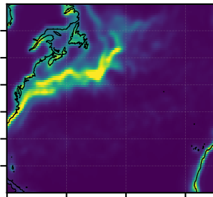
(f) mean_fill
