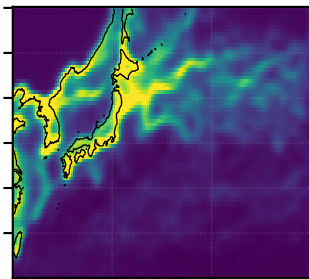
(f) mean_fill
