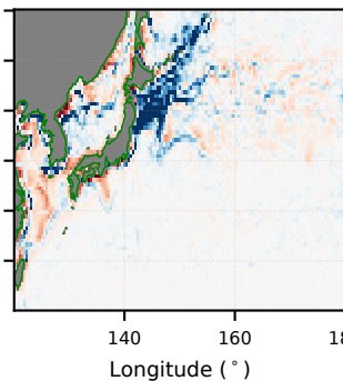
(f) mean_fill
