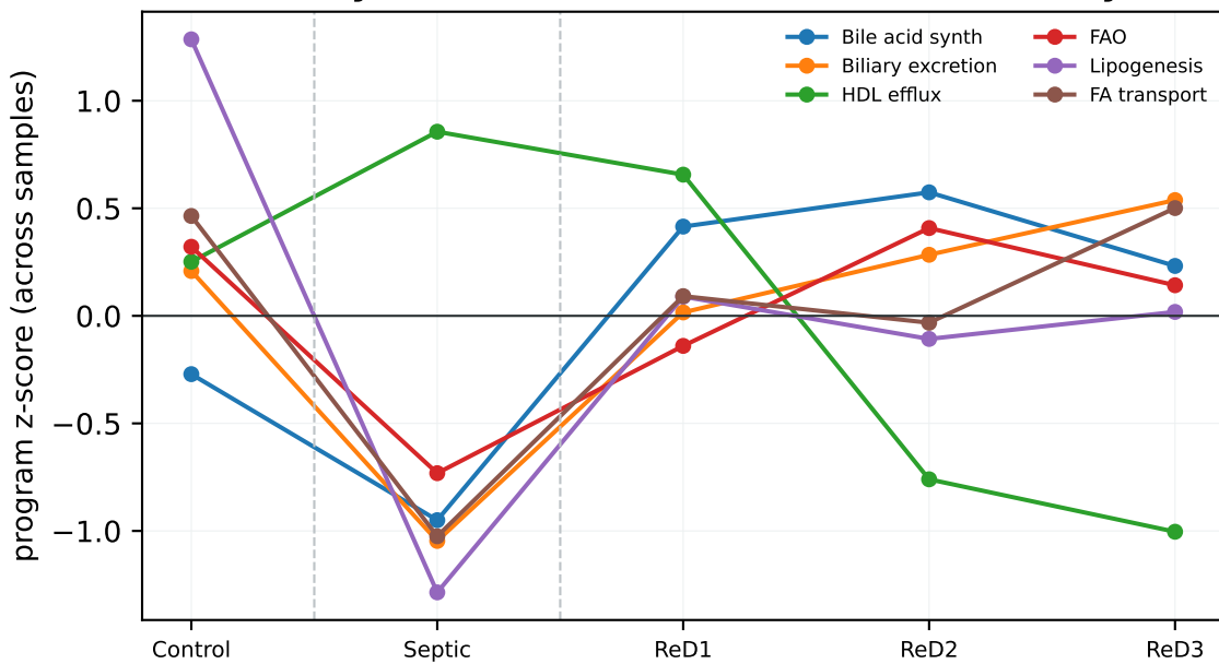
d Recovery after endotoxin removal (human only)
