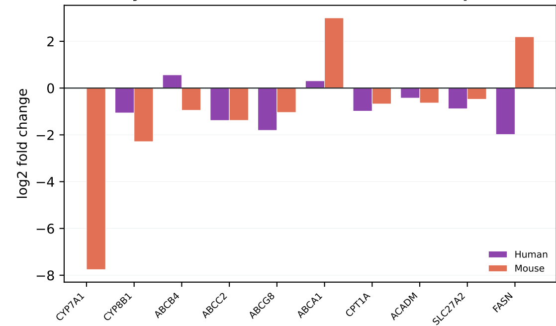
c Biliary axis vs ABCA1: conserved in both species
