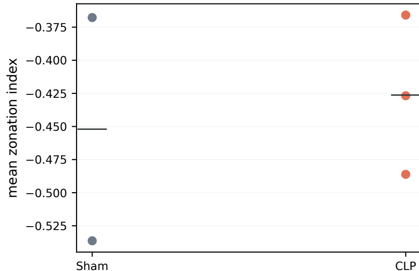
Per-sample means — no group difference
