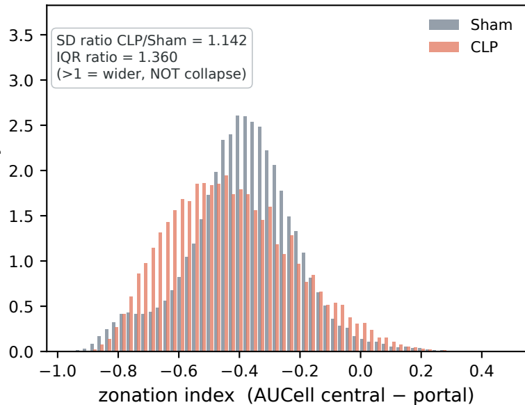
Zonation index distribution
