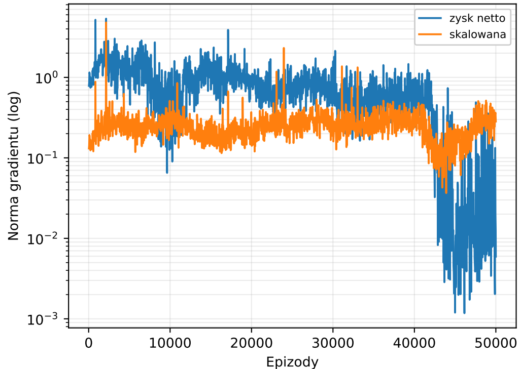
REINFORCE
