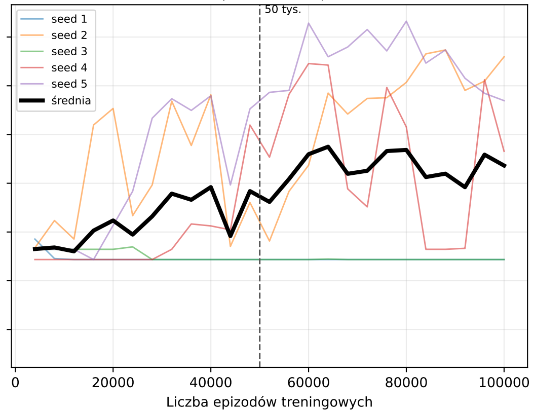
REINFORCE | FEATURES | skalowana
