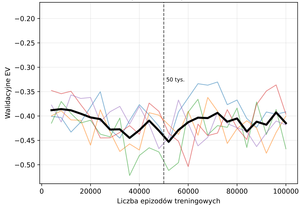
DQN | FEATURES | zysk netto
