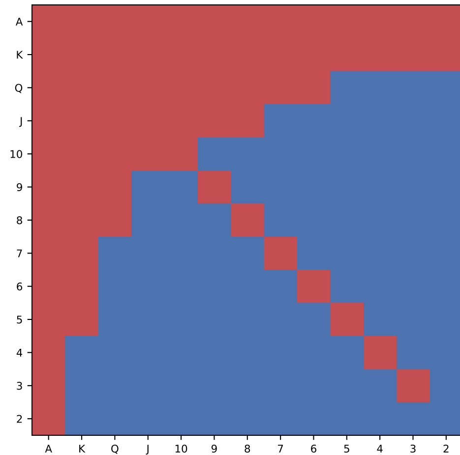
RuleBased
