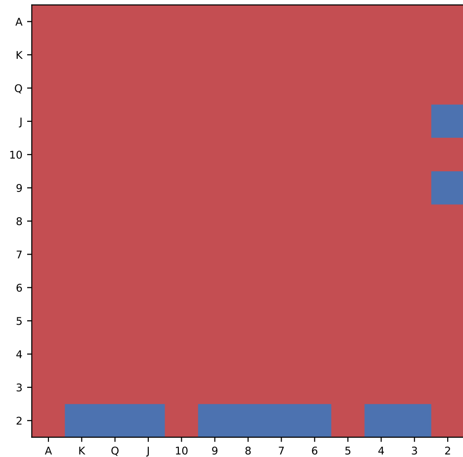
REINFORCE
