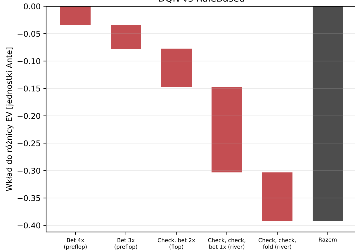
DQN vs RuleBased
