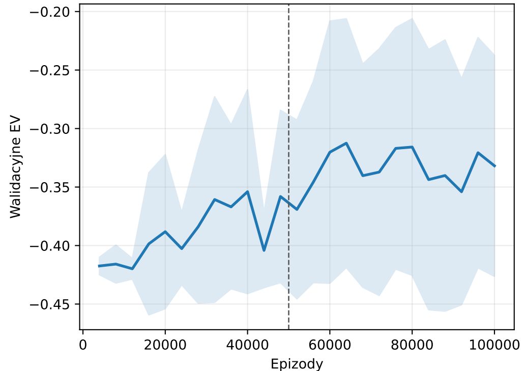
REINFORCE | FEATURES | skalowana
