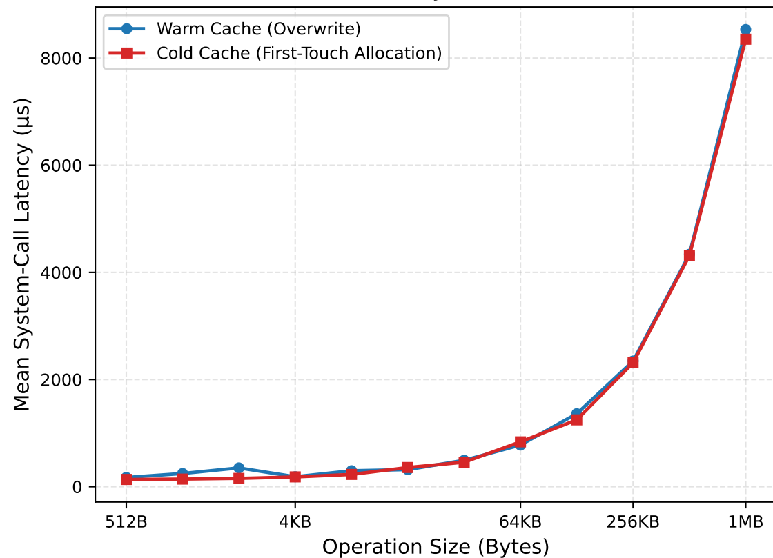
(a) Write Latency: Cold vs. Warm
