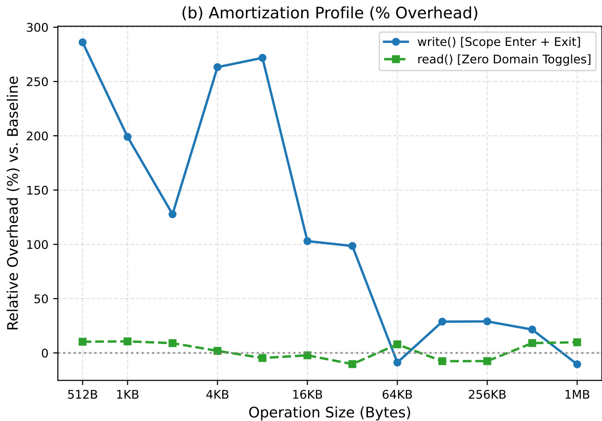
Figure 1: Unified Multi-Syscall Amortization Curves (Warm Cache)
