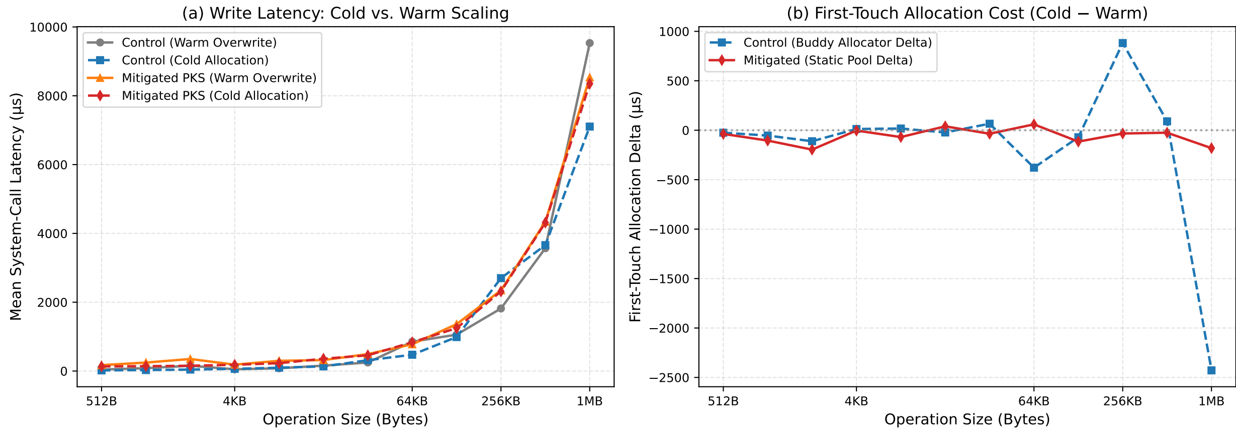
Figure 2: Cold vs. Warm Cache Scaling (Allocator Overhead Isolation)
