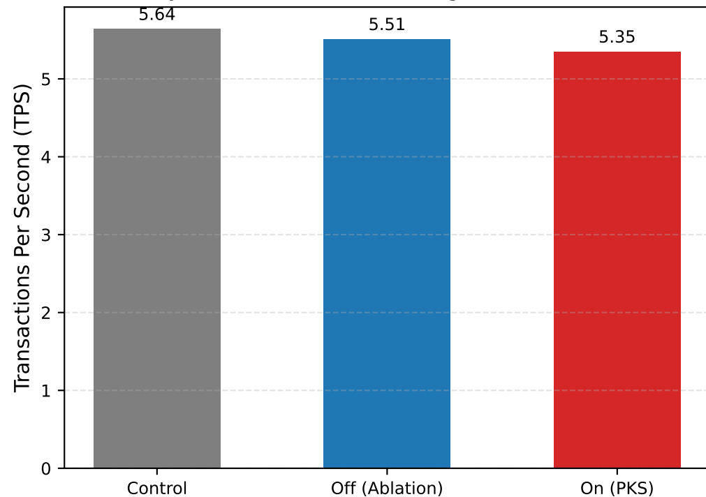
(a) synchronous=FULL (Storage Flush Bounded)
