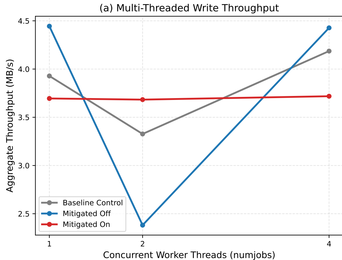
Figure 4: Multi-Core Concurrency Scaling
