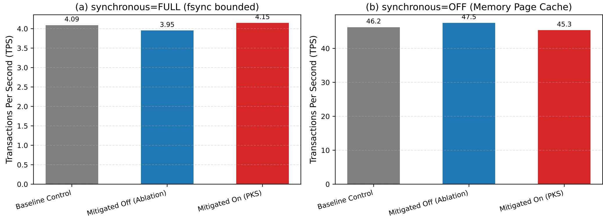
Figure 5: SQLite Macrobenchmark (Rollback Journal Mode)
