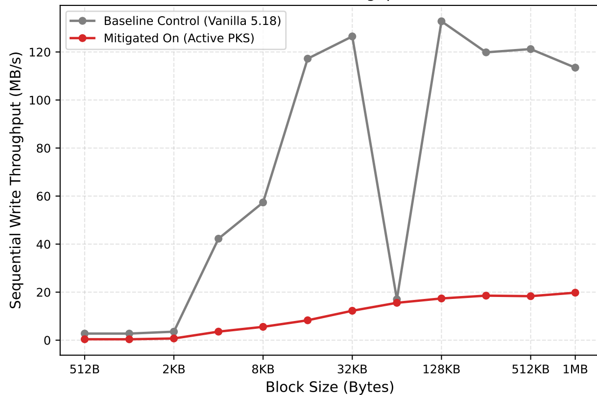
(a) Write Throughput
