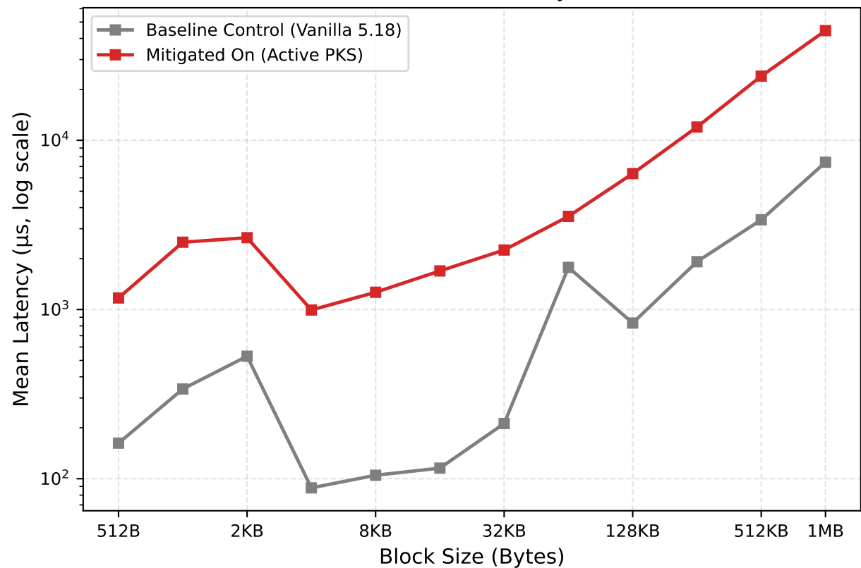
(b) Write Latency
