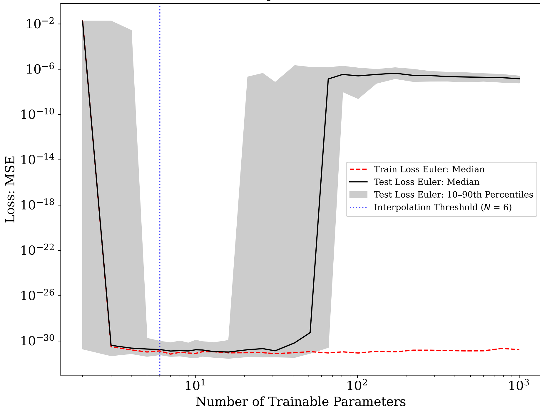
LQ, RF Min-Norm (lstsq, ReLU), N = 6 : Train vs Test Loss
