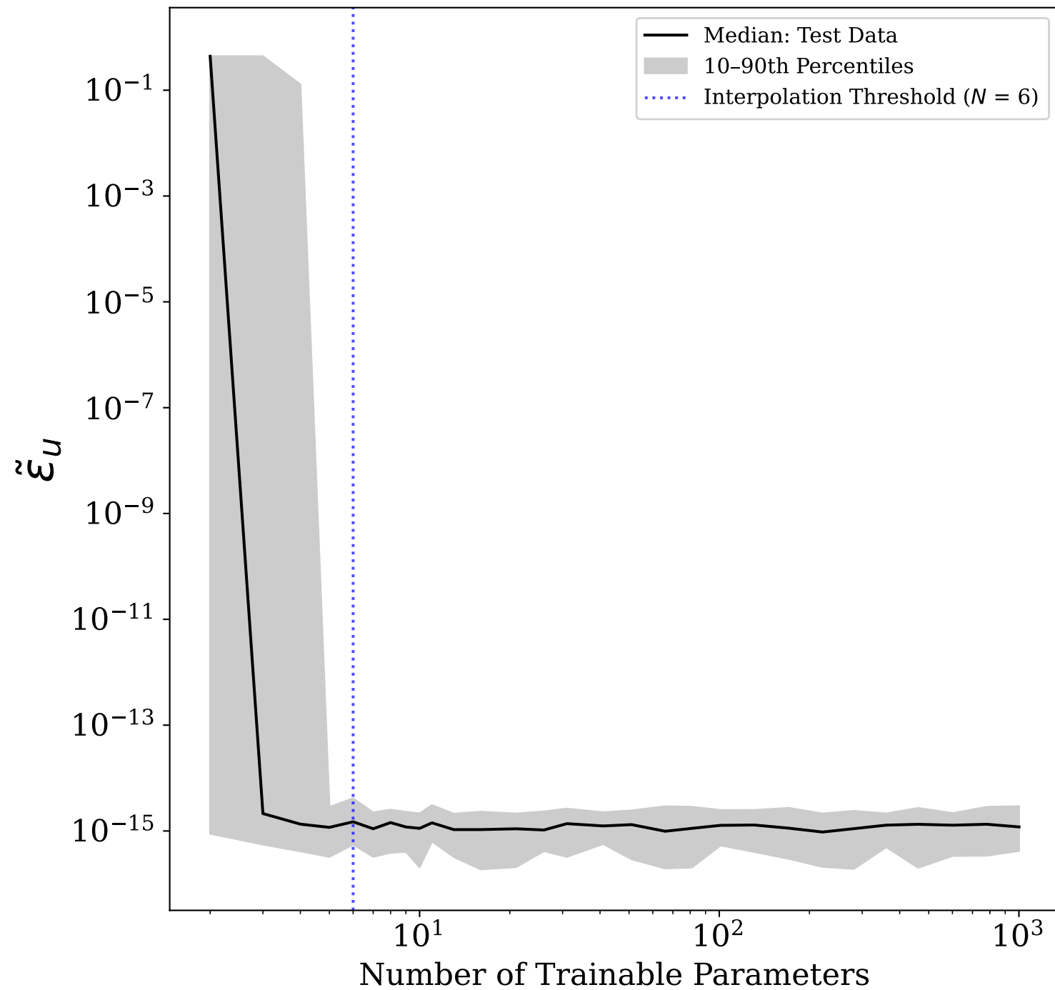
LQ, RF + interior-TV ( \lambda = 1 , ReLU), N = 6 : Median Abs Relative Error
