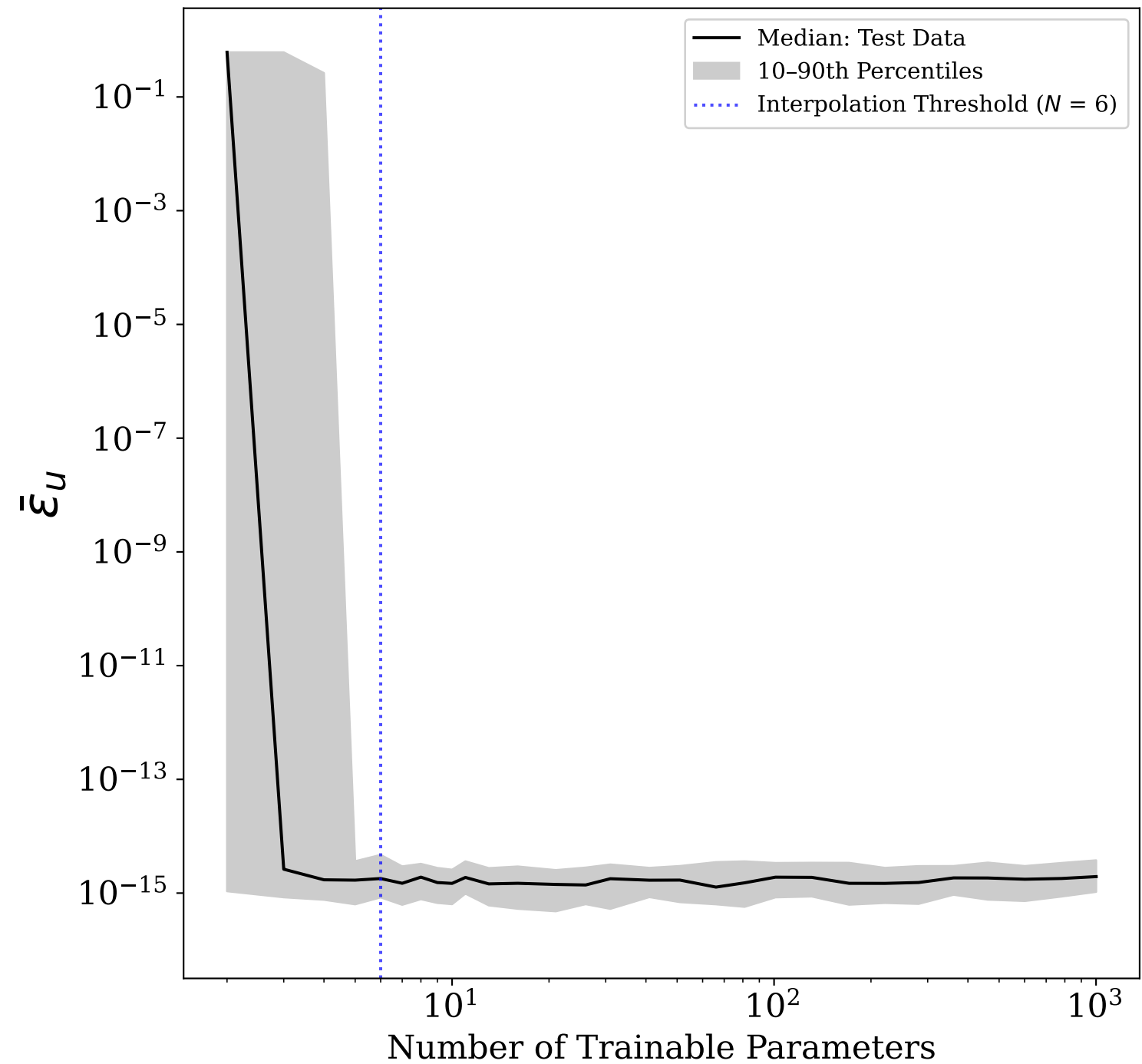
LQ, RF + interior-TV ( \lambda = 1 , ReLU), N = 6 : Max Abs Relative Error
