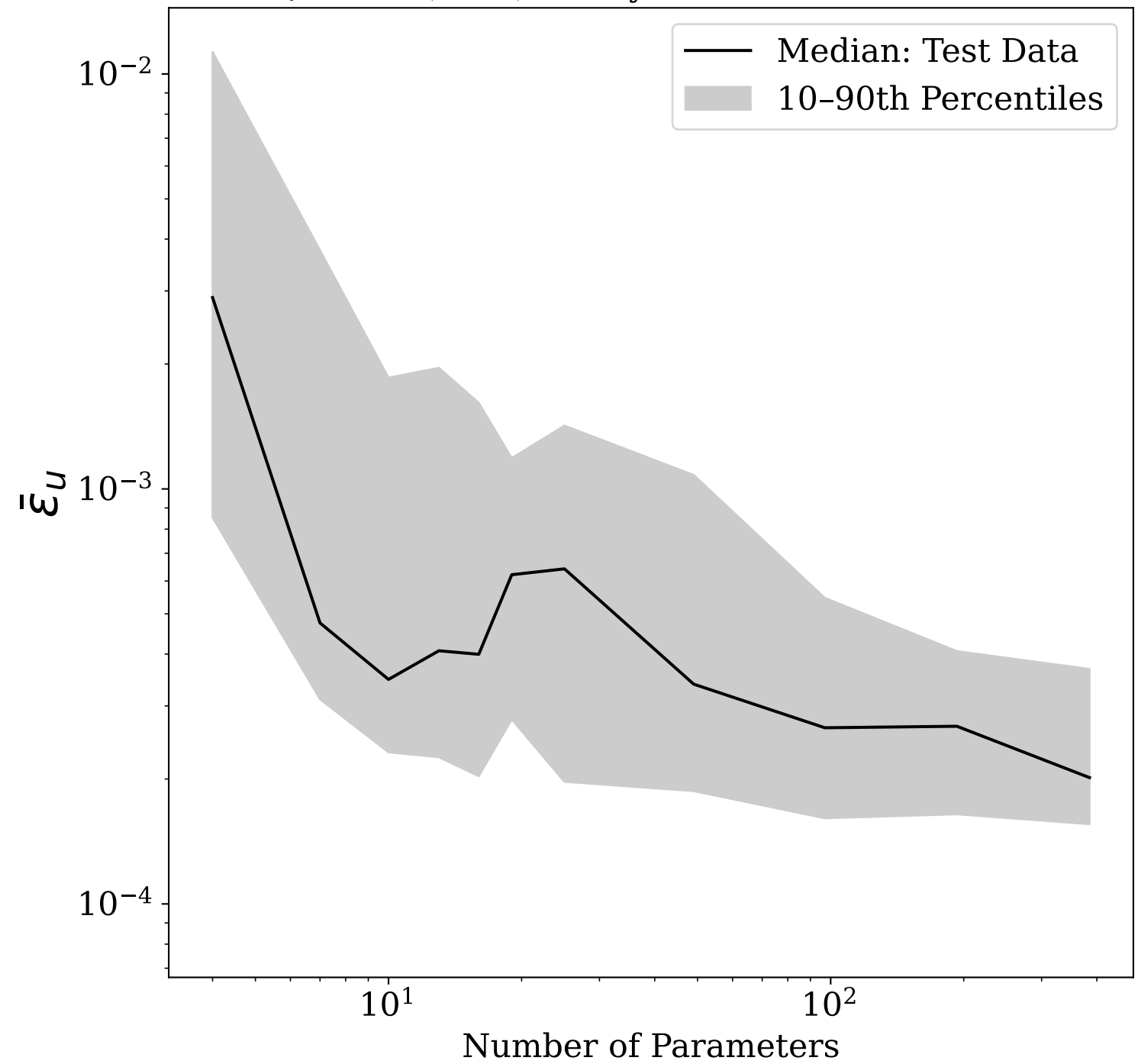
LQ Model (Tanh): Policy, Max Abs Relative Error
