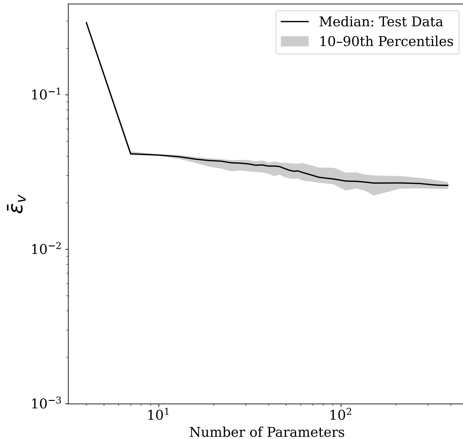
McCall Model: Max Abs Relative Error
