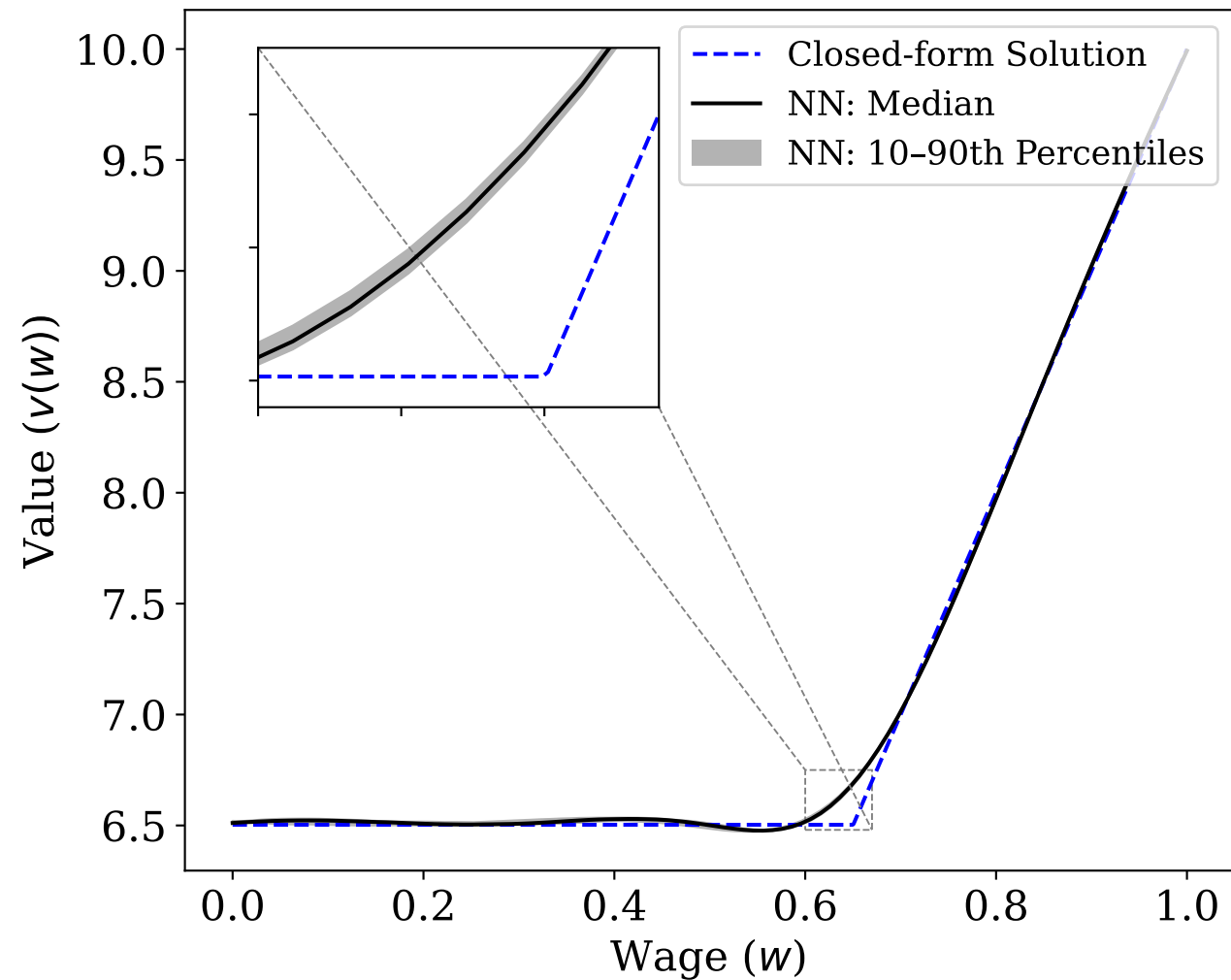
McCall Model: Closed-form vs NN ( H = 128 )
