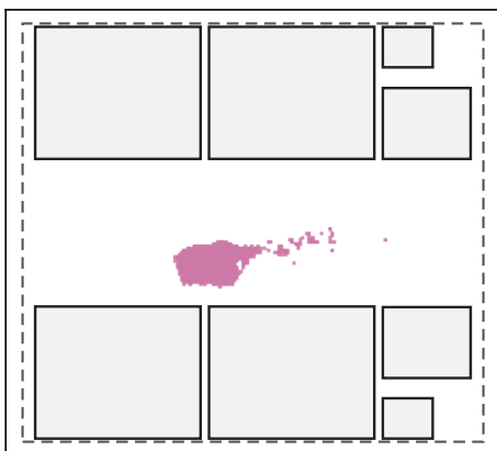
Memory scrub engine 1,173 instances
