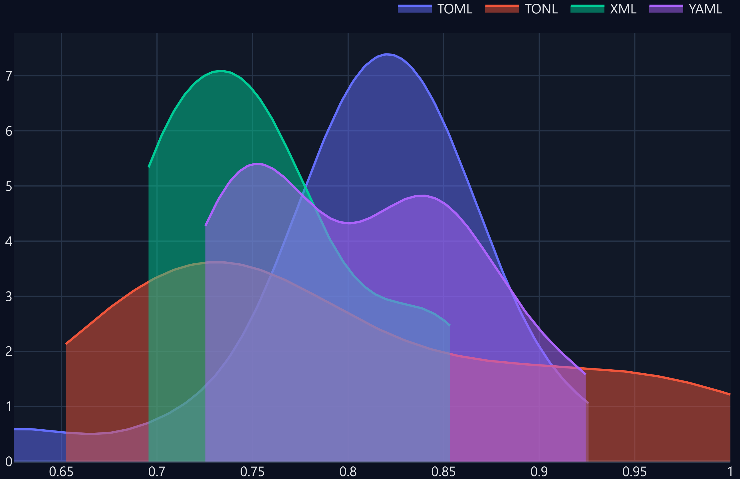
semantic_score KDE distribution
