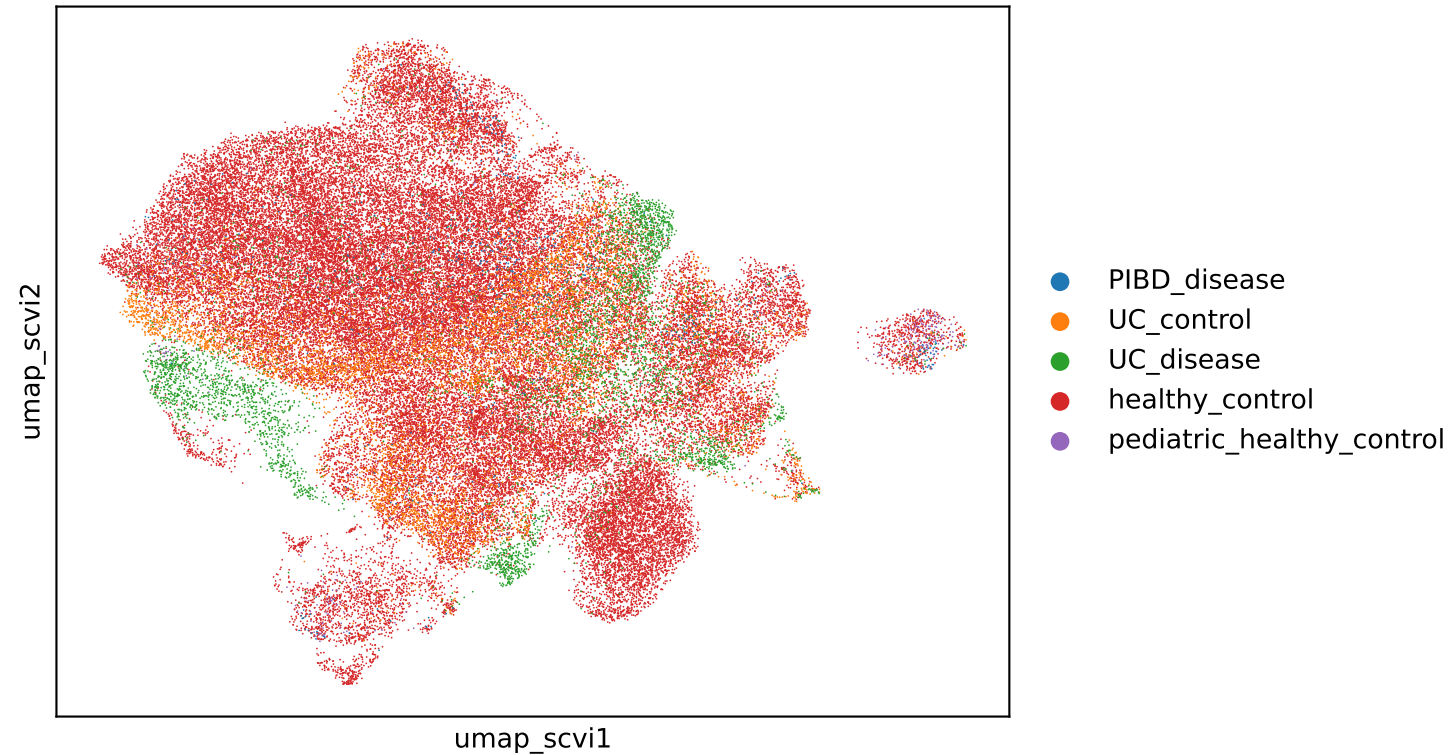
donor_disease_category (scvi)
