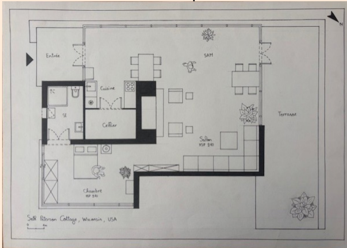
Seth Peterson Cottage, Wisconsin, USA
