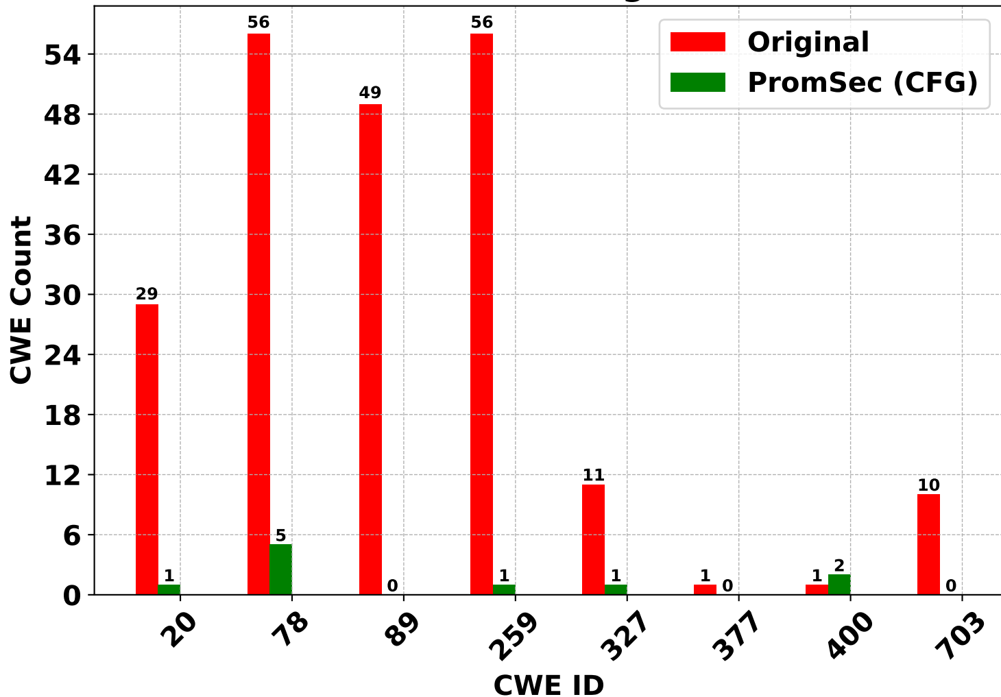
CWE ID Histogram
