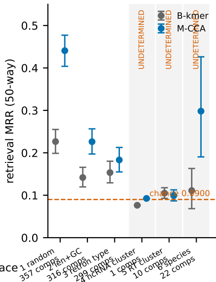
b The candidate ladder
