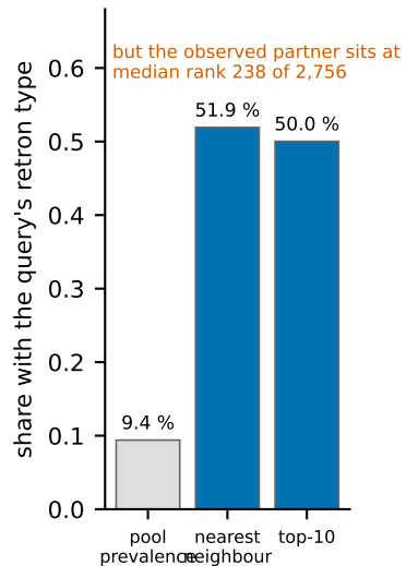
c 5.32x type enrichment
