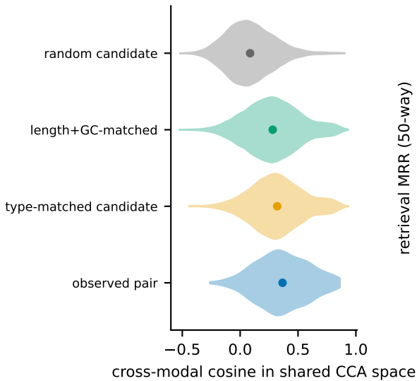
a Similarity by candidate class
