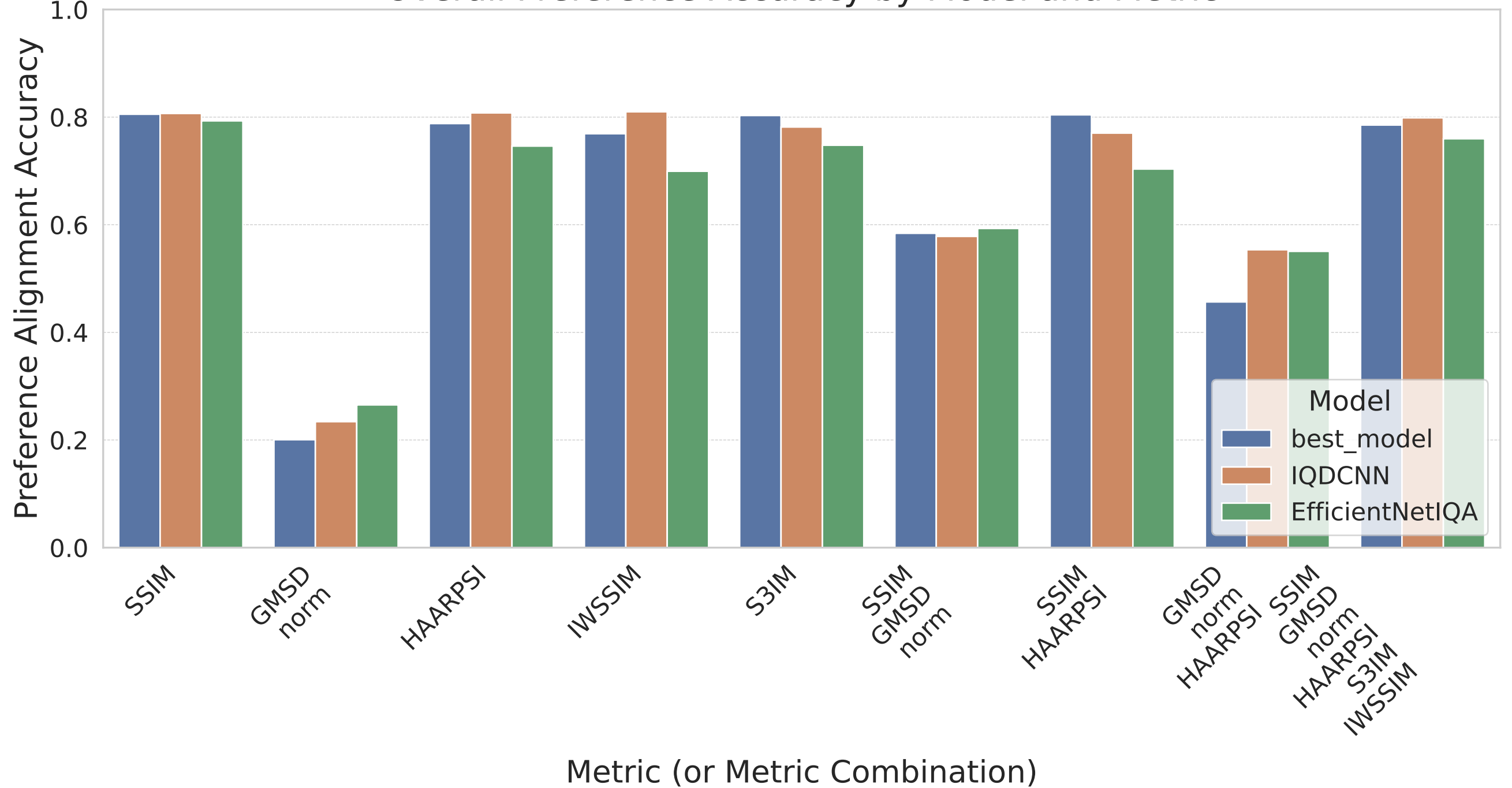
Overall Preference Accuracy by Model and Metric
