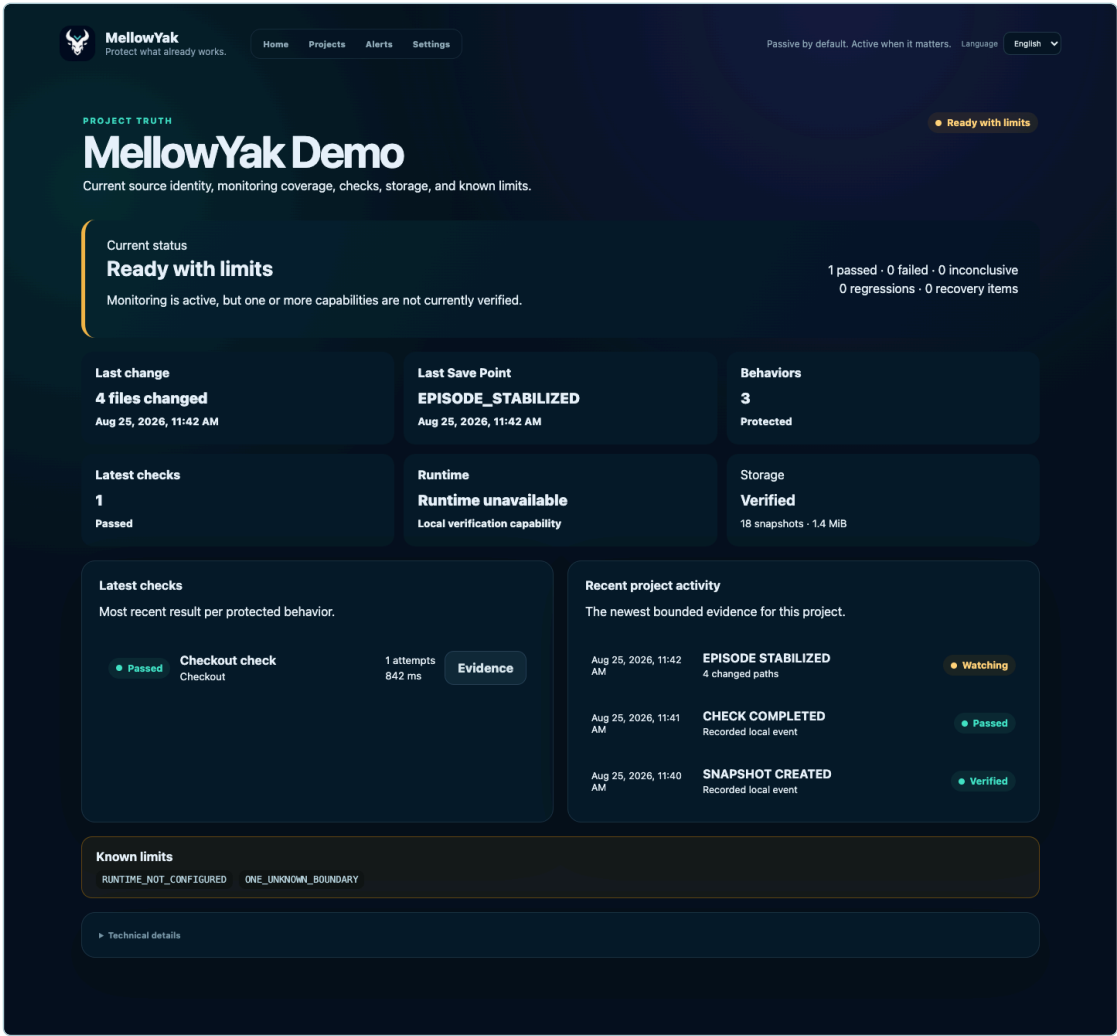
Project Overview Ready With Limits
