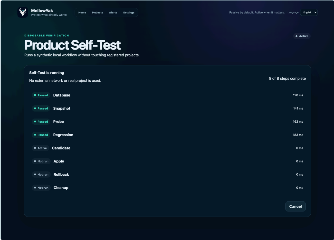
Self Test Running
