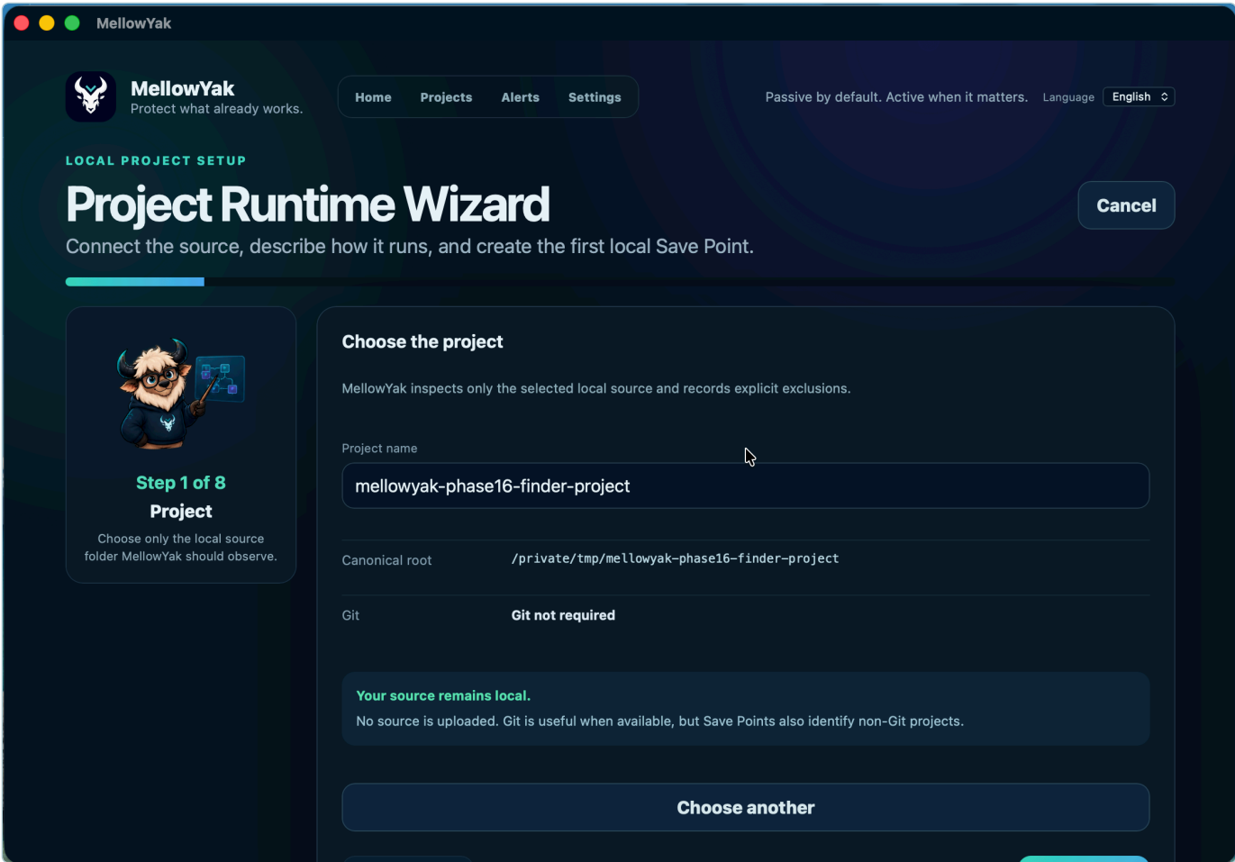
Finder Alias Canonical Resolution
