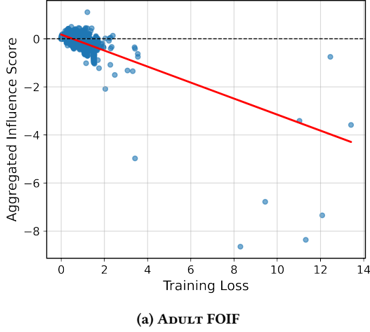
Figure 4: The Loss vs Influence Plot with regression line for the FOIF and TracIn for the full size ADULT dataset.
