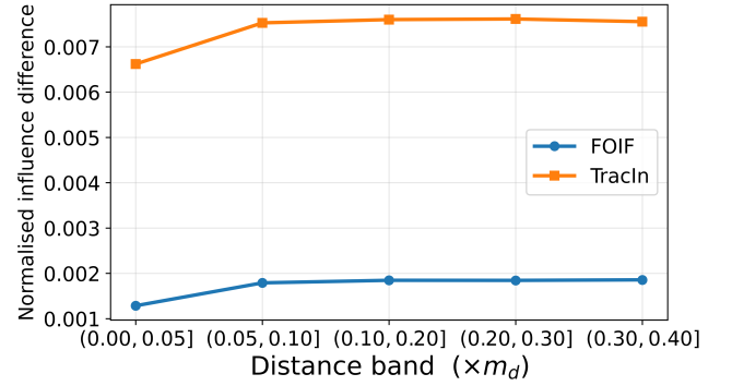
Figure 5: Normalised mean absolute influence-score difference across distance bands for FOIF and TracIn on DIAMONDS. Distance bands are expressed as multiples of the maximum pairwise distance m_d .
