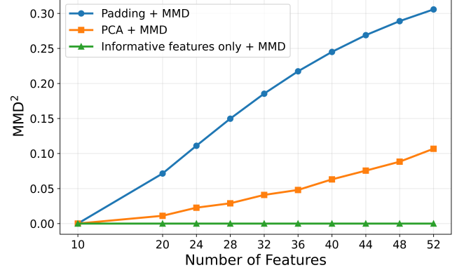
Figure 2: Maximum Mean Discrepancy (MMD) measured under three different dataset representations as the number of features increases. Smaller MMD values indicate greater distributional similarity.
