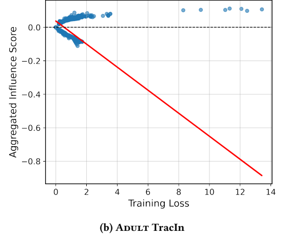
Figure 4: The Loss vs Influence Plot with regression line for the FOIF and TracIn for the full size ADULT dataset.
