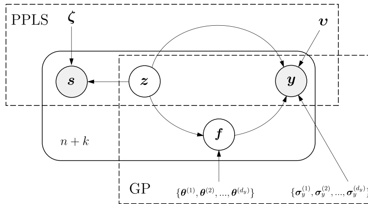
Figure 4. Graphical model for the k^{\text{th}} adaptive sampling iteration of PPLS-BO with a training data set \mathcal{D} of size n + k with (random) design variables \mathbf{s} and observations \mathbf{y} = (y^{(1)} y^{(2)} \dots y^{(d_y)}) . Unobserved latent variables \mathbf{z} and hyperparameters \zeta = \{\mathbf{W}, \hat{\Sigma}_s\} and \mathbf{v} = \{\mathbf{Q}, \hat{\Sigma}_y\} are learned using PPLS independent from the GP surrogates with target output variables \mathbf{f} = (f^{(1)} f^{(2)} \dots f^{(d_y)}) and GP hyperparameters \{\theta^{(1)}, \theta^{(2)}, \dots, \theta^{(d_y)}\} and \{\sigma_y^{(1)}, \sigma_y^{(2)}, \dots, \sigma_y^{(d_y)}\} .
