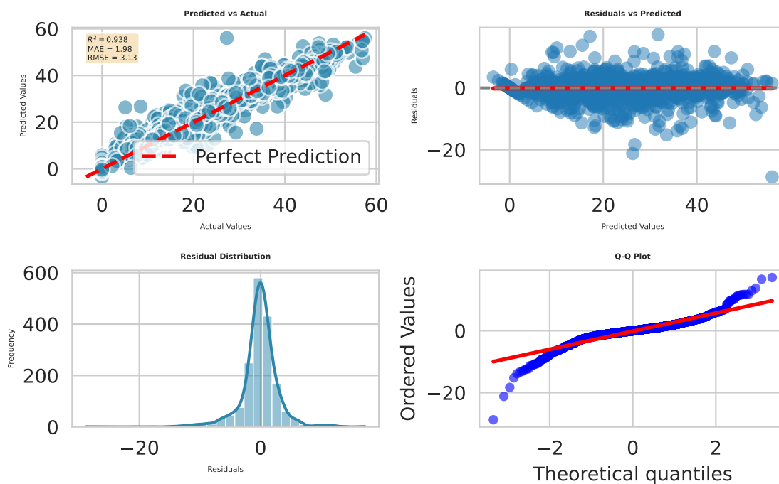
Gradient Boosting (MSE)
