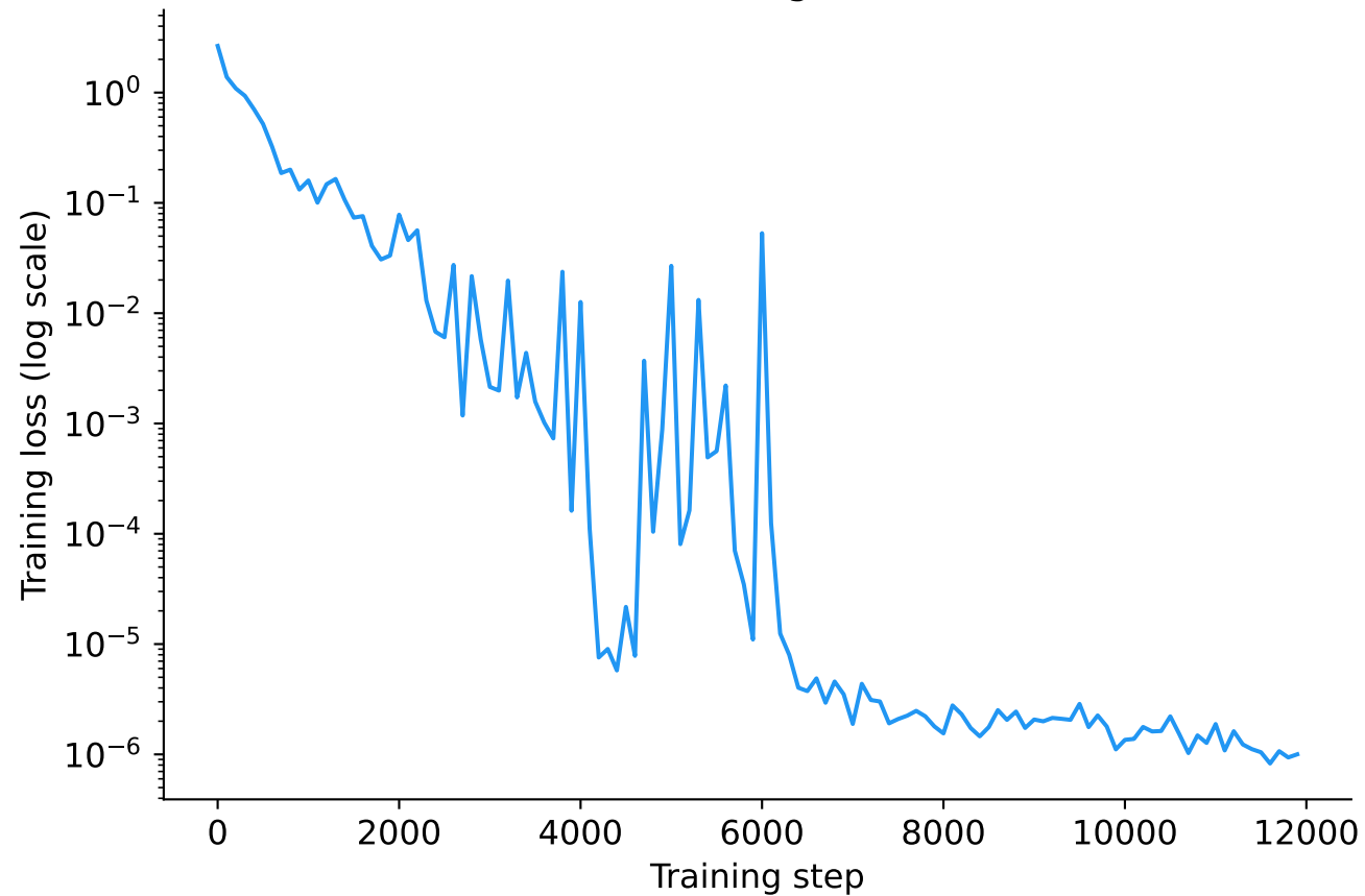
A. Training Loss
