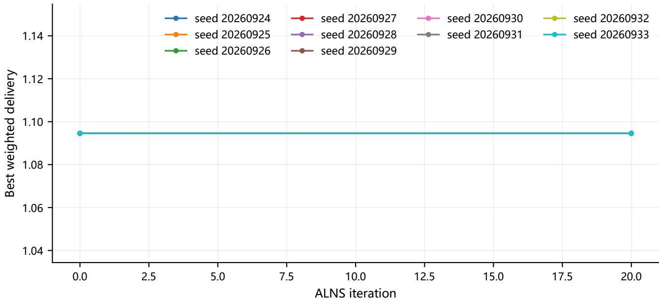
ALNS convergence
