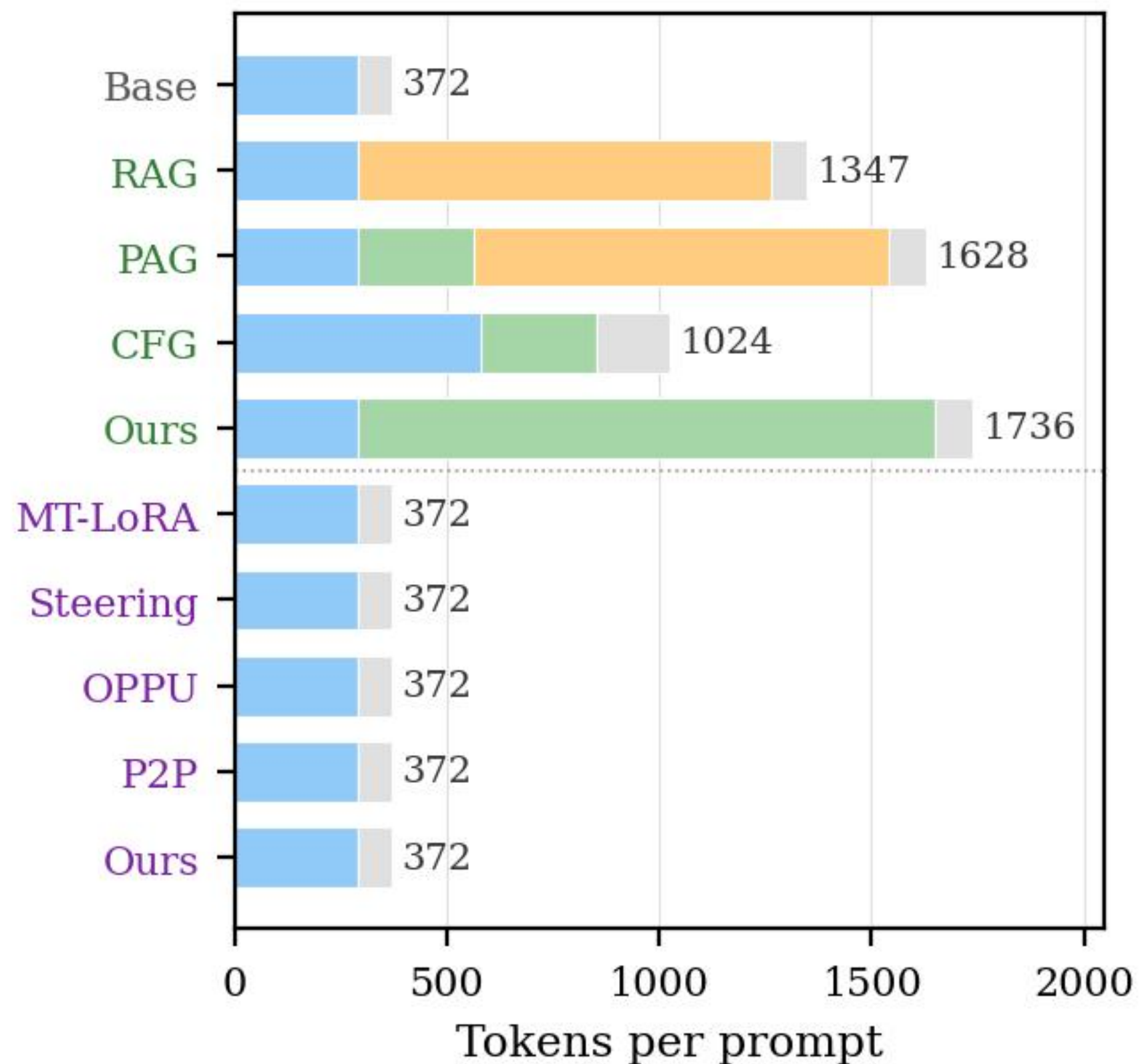
Long-Dialogue
