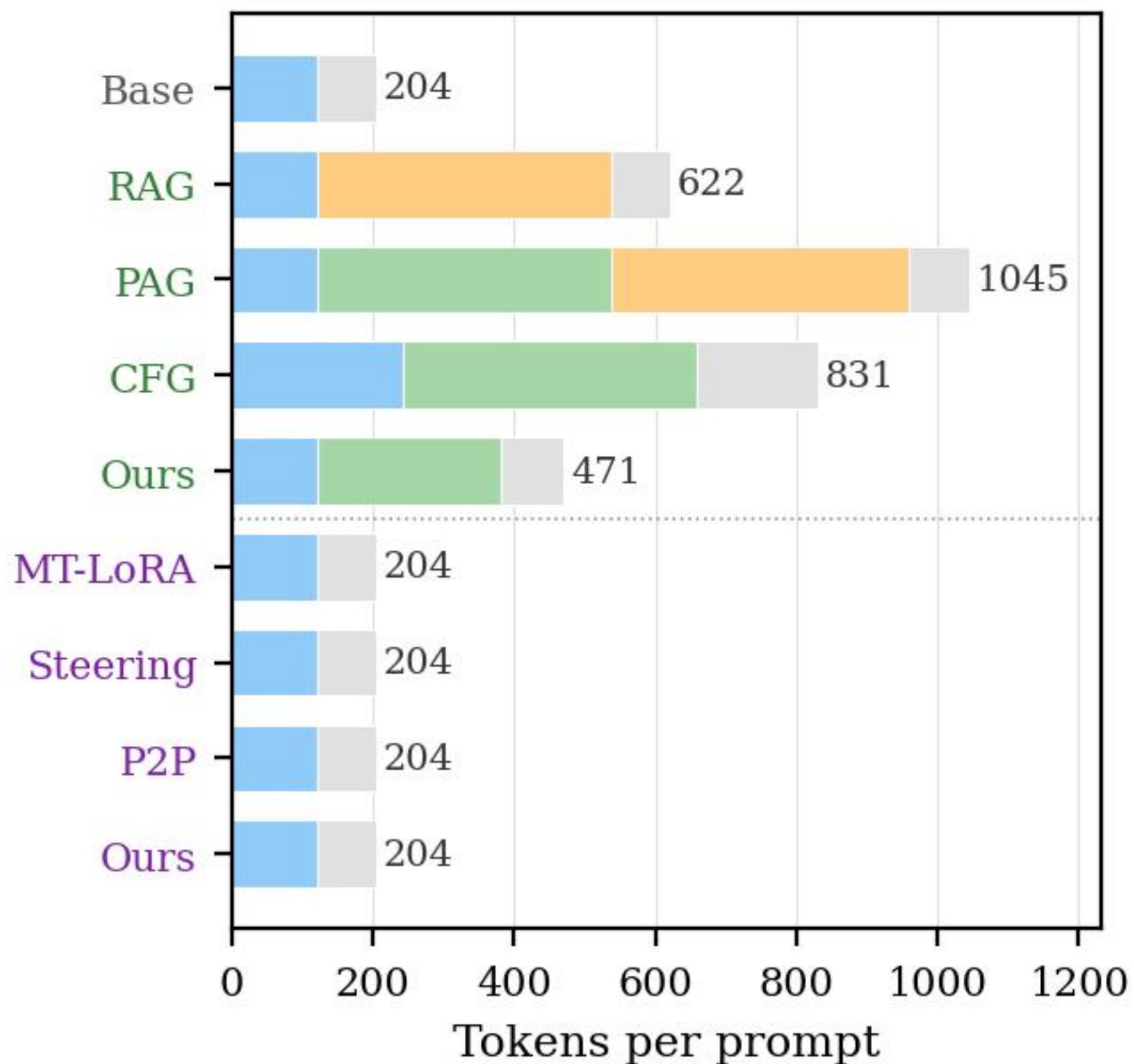
Short-Dialogue
