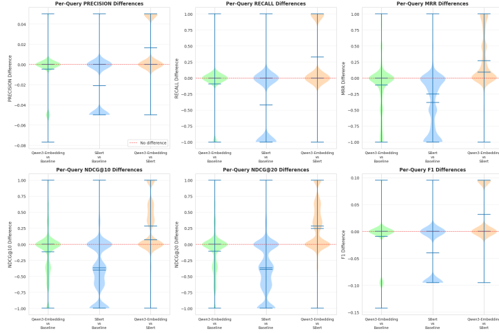
Figure 42: Per-query metric differences for Timeline QA sparse configuration.
