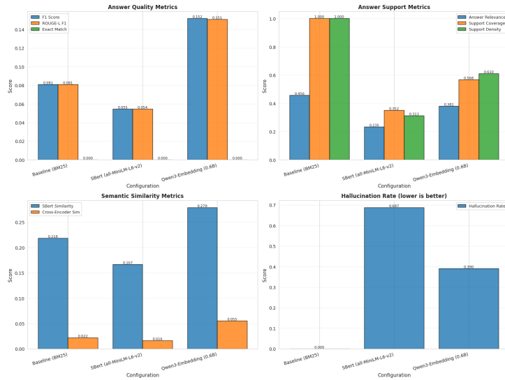
Figure 31: Generation metrics comparison for Timeline QA dense configuration.
