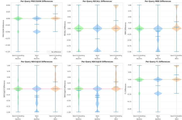
Figure 30: Per-query metric differences for Timeline QA dense configuration.
