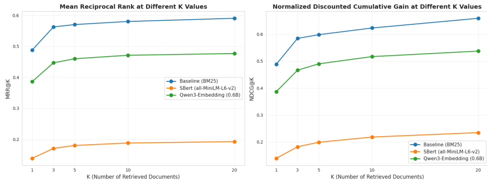
Figure 35: MRR and NDCG at different K values for Timeline QA medium configuration.
