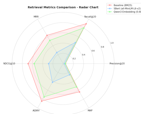
Figure 40: Radar chart showing all retrieval metrics for Timeline QA sparse configuration.
