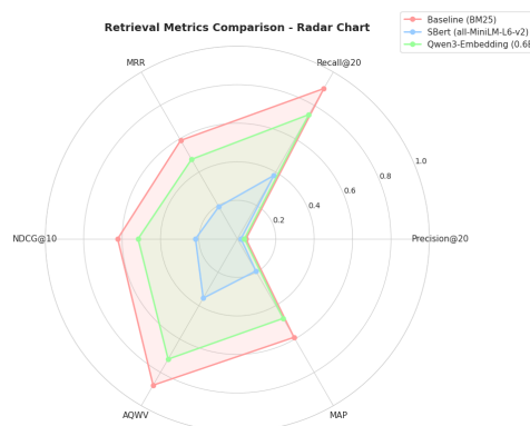
Figure 34: Radar chart showing all retrieval metrics for Timeline QA medium configuration.
