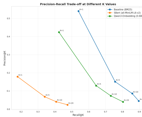
Figure 39: Precision-recall trade-off at different K values for Timeline QA sparse configuration.
