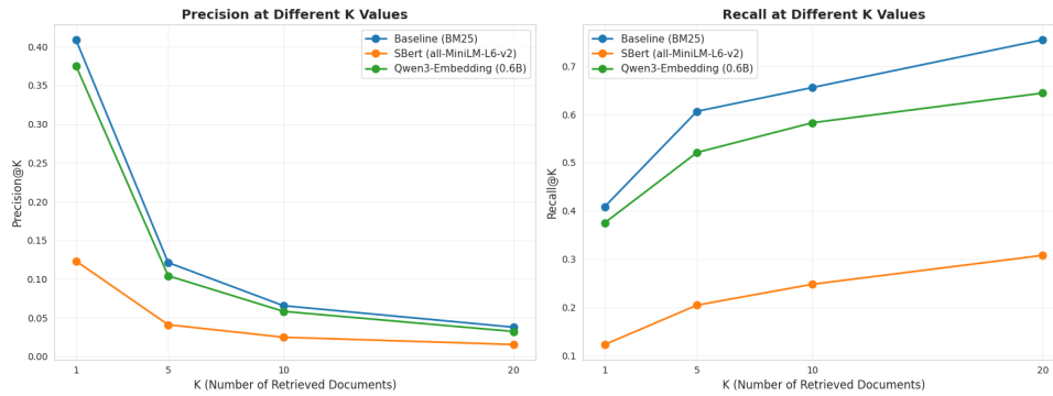
Figure 26: Precision and recall at different K values for Timeline QA dense configuration.
