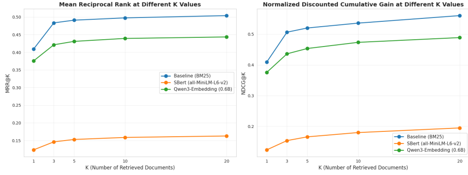
Figure 29: MRR and NDCG at different K values for Timeline QA dense configuration.
