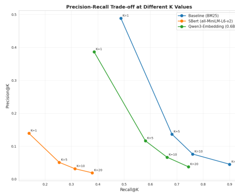
Figure 33: Precision-recall trade-off at different K values for Timeline QA medium configuration.
