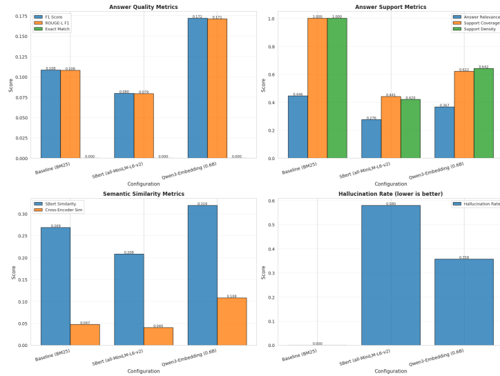
Figure 43: Generation metrics comparison for Timeline QA sparse configuration.
