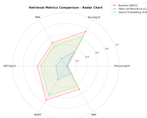
Figure 28: Radar chart showing all retrieval metrics for Timeline QA dense configuration.
