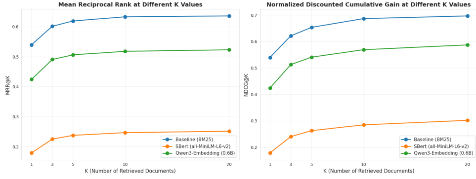
Figure 41: MRR and NDCG at different K values for Timeline QA sparse configuration.
