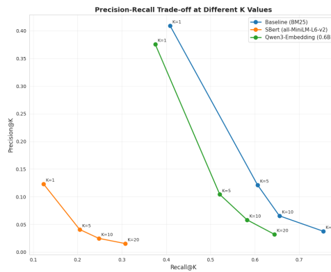
Figure 27: Precision-recall trade-off at different K values for Timeline QA dense configuration.
