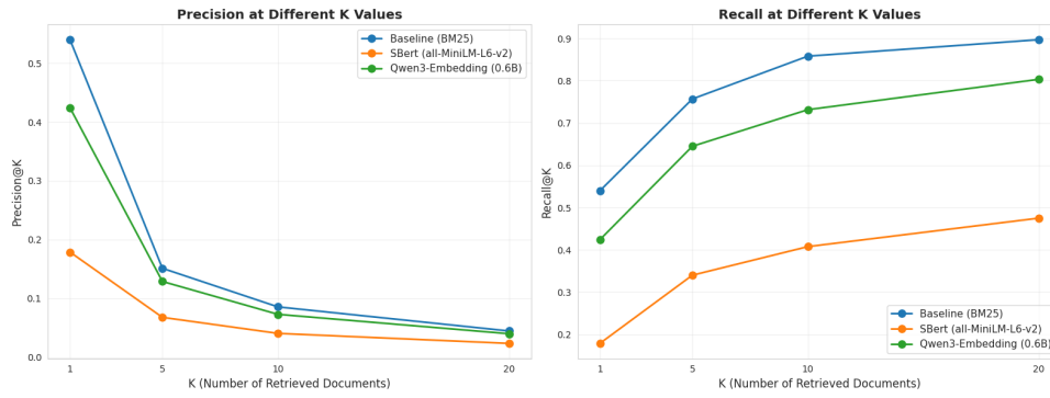
Figure 38: Precision and recall at different K values for Timeline QA sparse configuration.
