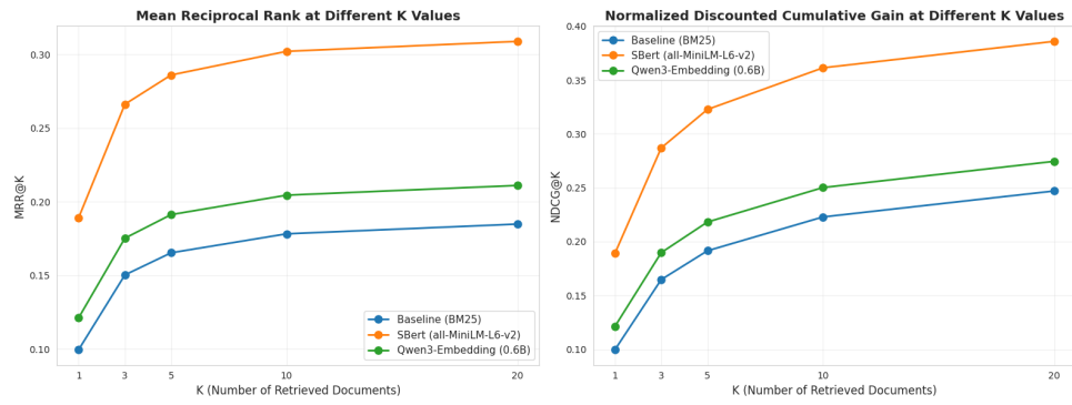
Figure 11: MRR and NDCG at different K values for MS MARCO passage evaluation.
