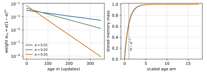
FIG. 2. Exponential memory weights generated by Eq. (4). A contribution of age m enters with weight w_m = \alpha(1 - \alpha)^m . When ages are measured in the scaled variable \alpha m , the accumulated memory weight collapses onto a persistence scale of order \alpha^{-1} updates.
