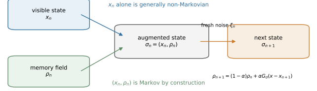
FIG. 1. Memory-state Markov embedding. The visible coordinate x_n is generally non-Markovian by itself, because the next update depends on the accumulated memory field \rho_n . Once \sigma_n = (x_n, \rho_n) is used as the state, all past influence enters through \rho_n , while fresh randomness enters through \xi_n .
