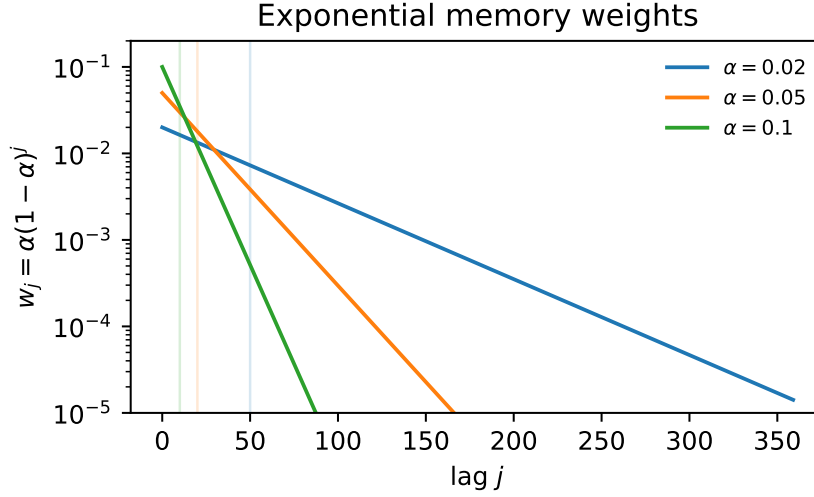
FIG. 1. Exponential memory weights w_j = \alpha(1 - \alpha)^j . Vertical guide lines mark j = \alpha^{-1} for each curve.
