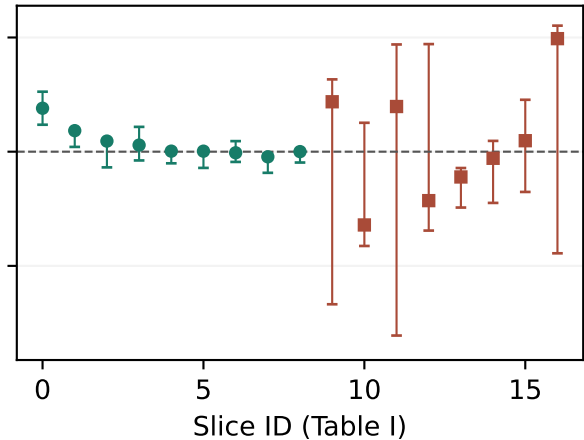
(b) Position-relative RMS
