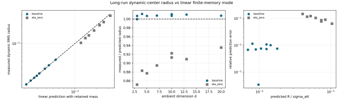
FIG. 3. Measured co-moving root-mean-square radii compared with the finite-memory linear prediction. Active slices remain close to the diagonal across run length and ambient dimension. The \eta = 0 controls are displayed separately because the active-force prediction is not an exact identity for their finite-window trace estimator.
