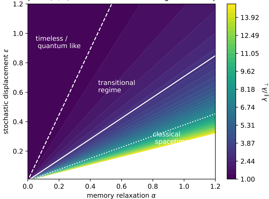
Phase Space ( \alpha , \varepsilon ): Direction of Time as Eigenvalue Separation
