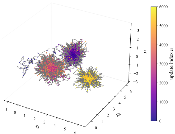
FIG. 1. Representative trajectory with multiple metastable knot-like regions. The line shows the visible trajectory, sampled points contribute to the memory density, and color denotes update index.
