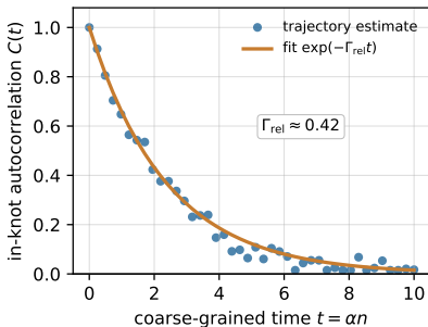
FIG. 4. Operational extraction of a knot relaxation rate from an in-knot autocorrelation. The decay of a coarse-grained observable C(t) over the intrinsic parameter t = \alpha n defines \tau_{\text{rel}} and hence \Gamma_{\text{rel}} = 1/\tau_{\text{rel}} . The figure is schematic: the diagnostic is the fitted relaxation scale, not the specific numerical value.
