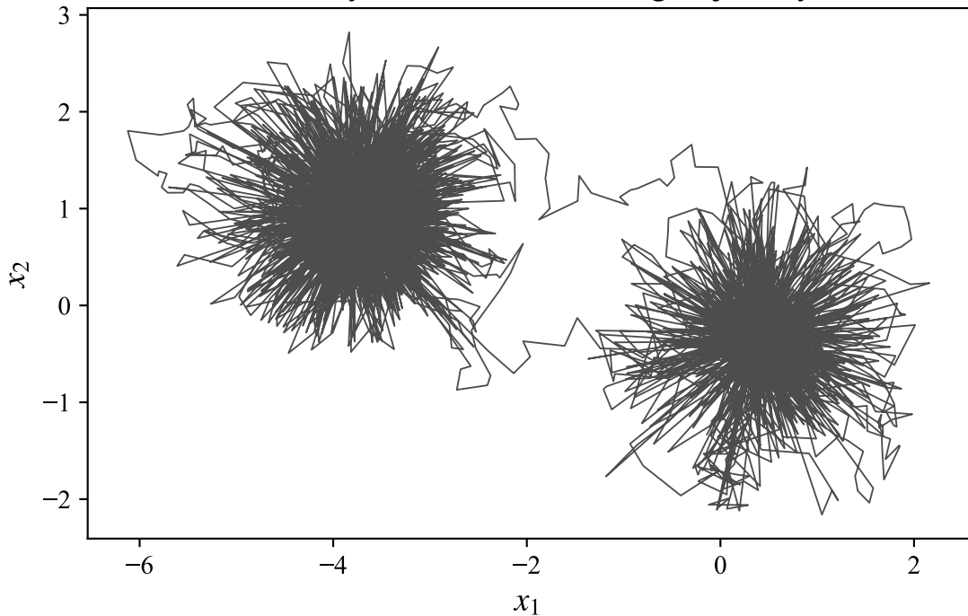
Memory-driven self-avoiding trajectory
