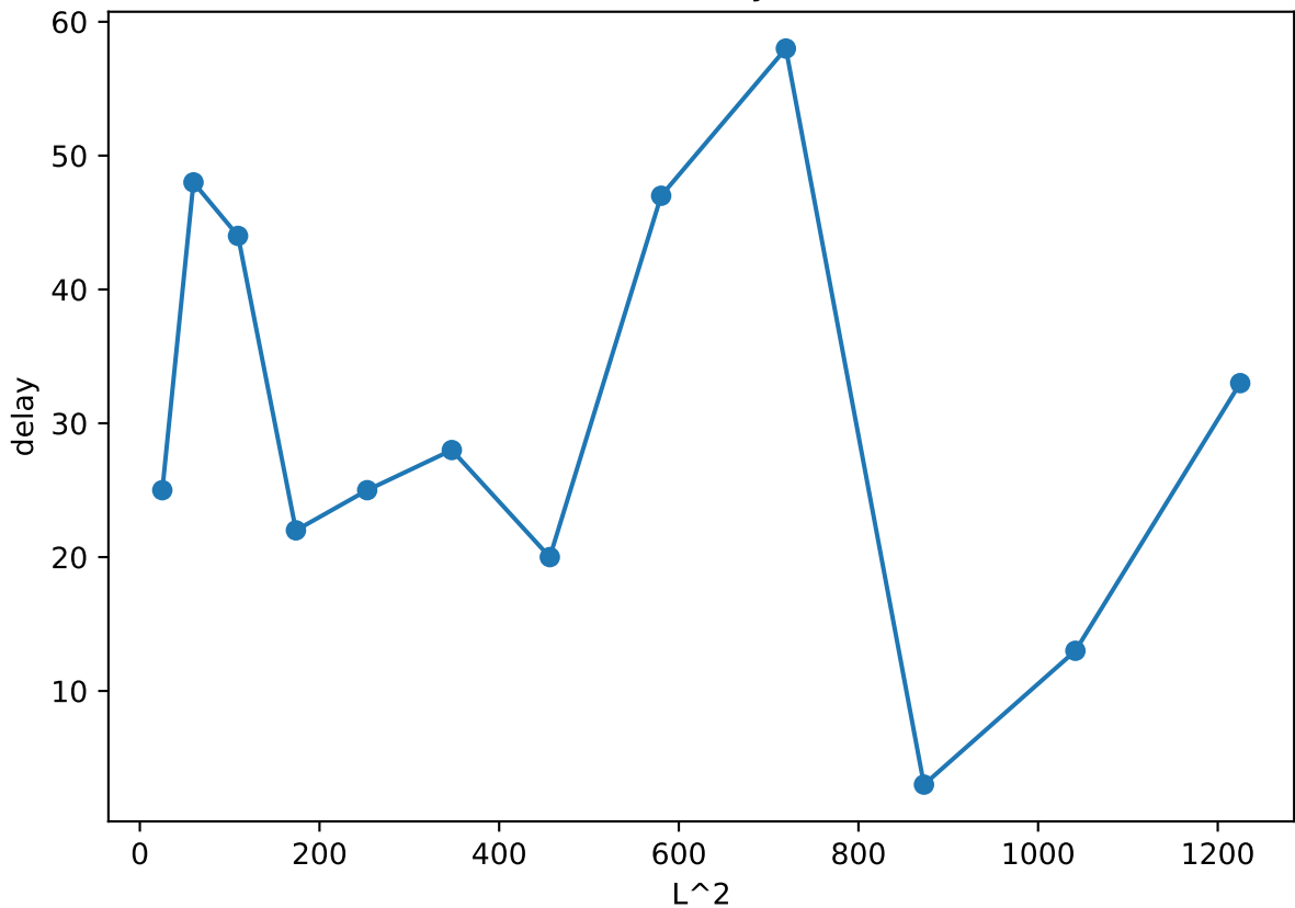
diffusive: Delay vs L^2
