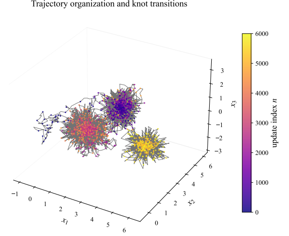
FIG. 1. Representative trajectory with multiple metastable knot-like regions. The line shows the visible trajectory, sampled points contribute to the memory density, and color denotes update index.
